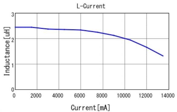
■ 1217AS-H-2R2N L-Current 20degC
